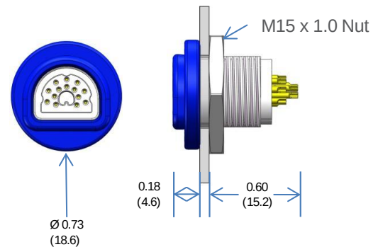
Front panel-mount (FPM) receptacle
