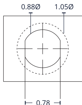
1.05p Mounting Flange Footprint
